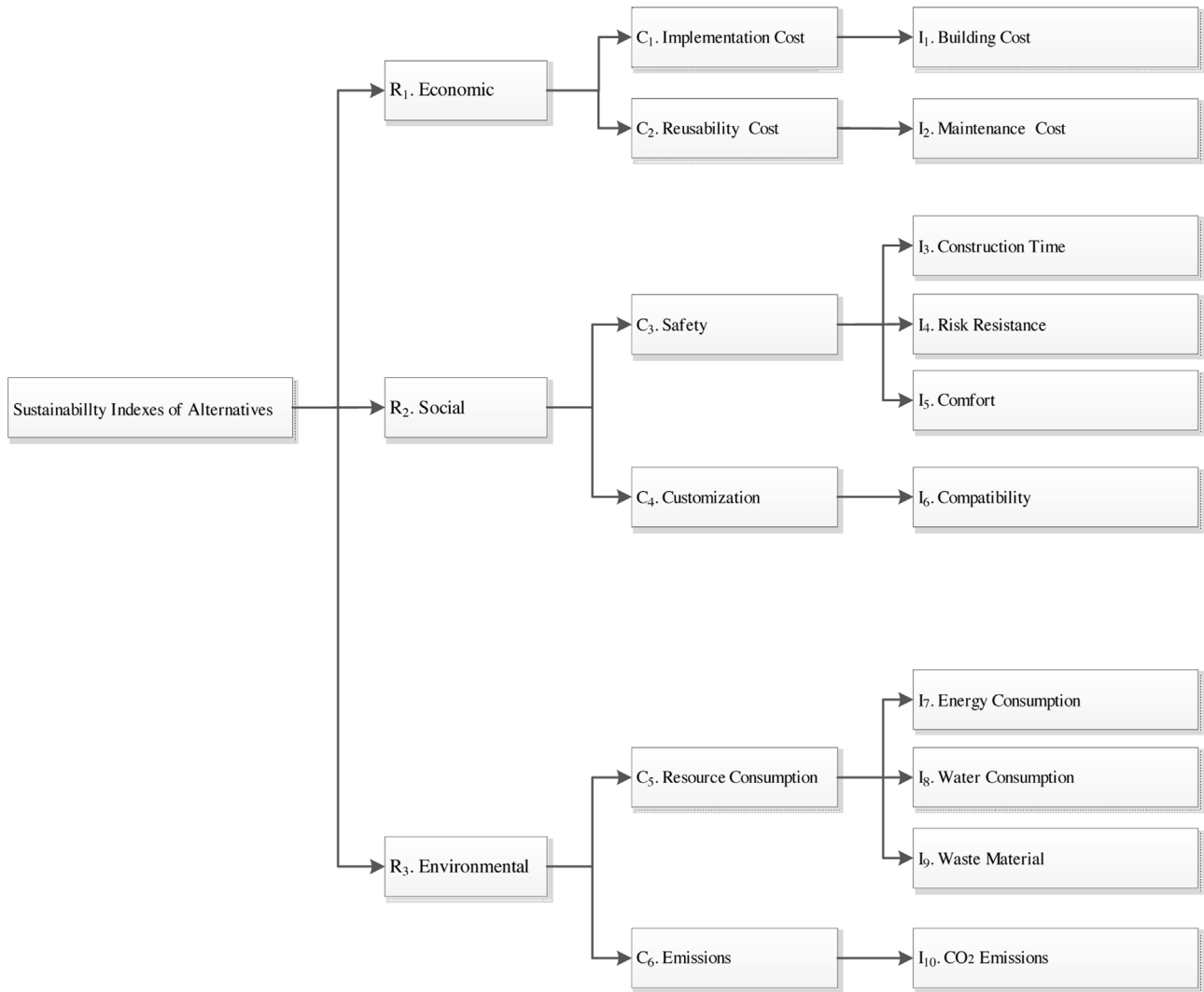
Fig. 4. Requirements tree designed for this model.
