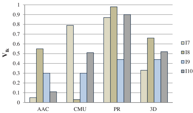
Fig. 8. Environmental indicator values for the four alternatives.
