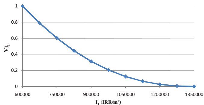
Fig. 6. Value function of building cost indicator ( I_1 ).
