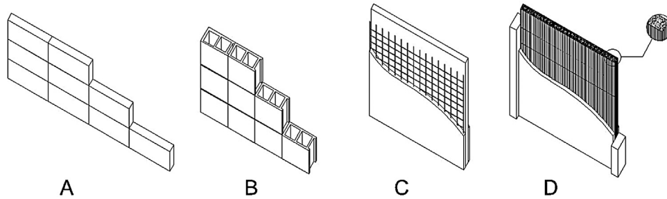
Fig. 3. View of the four wall technologies; (a) autoclaved aerated concrete block (AAC block), (b) concrete masonry unit (CMU), (c) pressed reeds panel, and (d) 3D sandwich panel wall.
