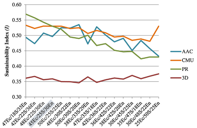
Fig. 9. Sustainability indexes of the four technologies with different requirement weights (economic (Ec), social (S), and environmental (En)).
